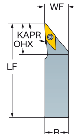
SVJBR/L-S 93.0°
