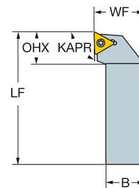
STGCR/L 91.0°
