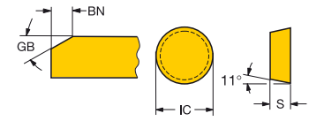
RPGN..S/T
