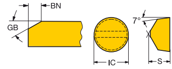
RCGX..K/T
