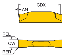
N123x2-CM
